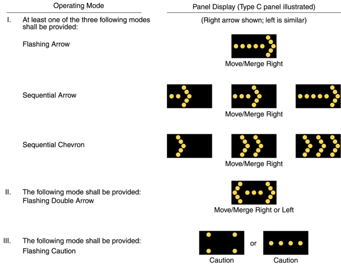
Figure 6F-3. Advance Warning Arrow Display Specifications
