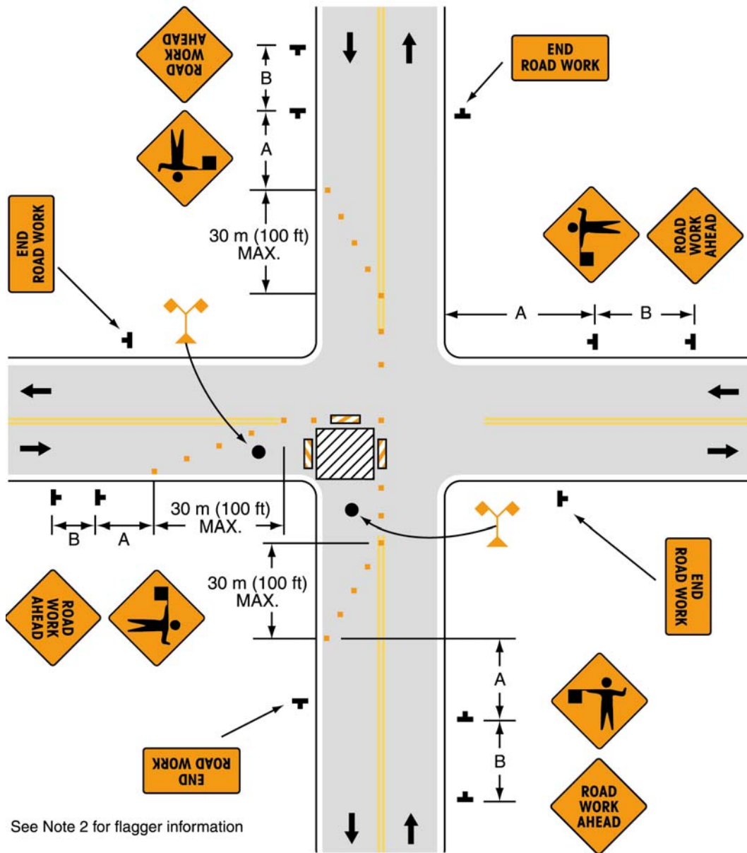
Typical Application 27
