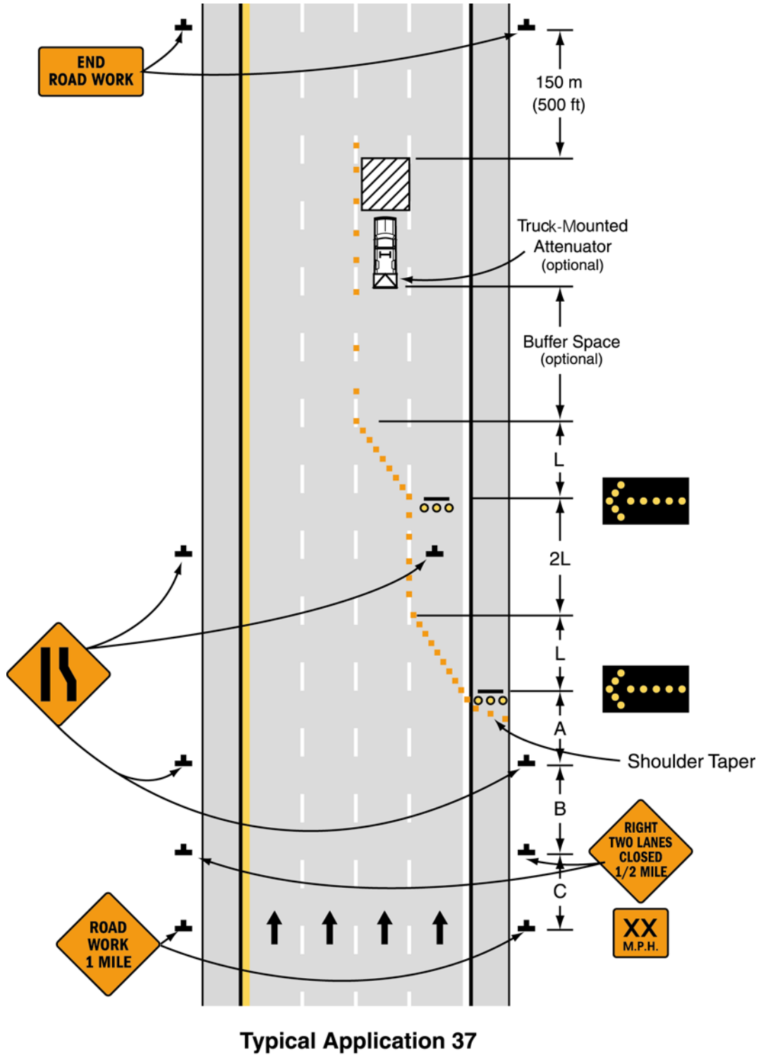
Figure 6H-37. Double Lane Closure on Freeway (TA-37)
