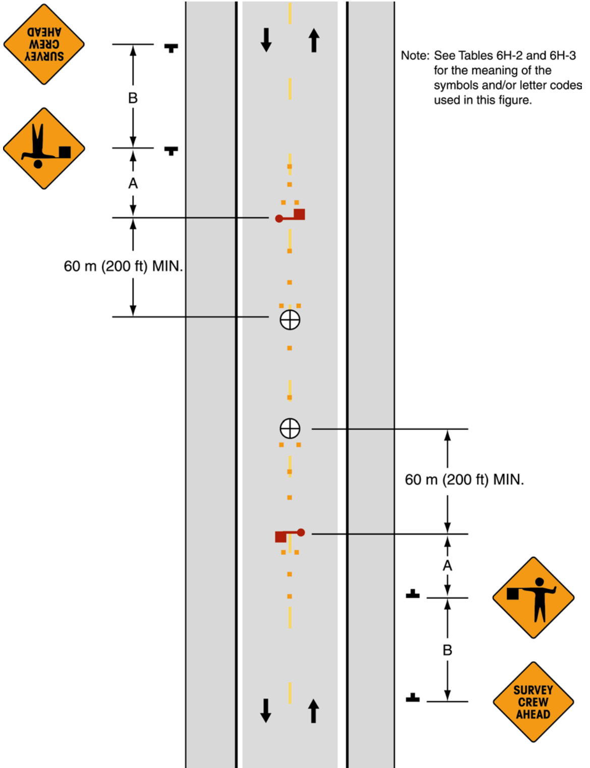
Typical Application 16
