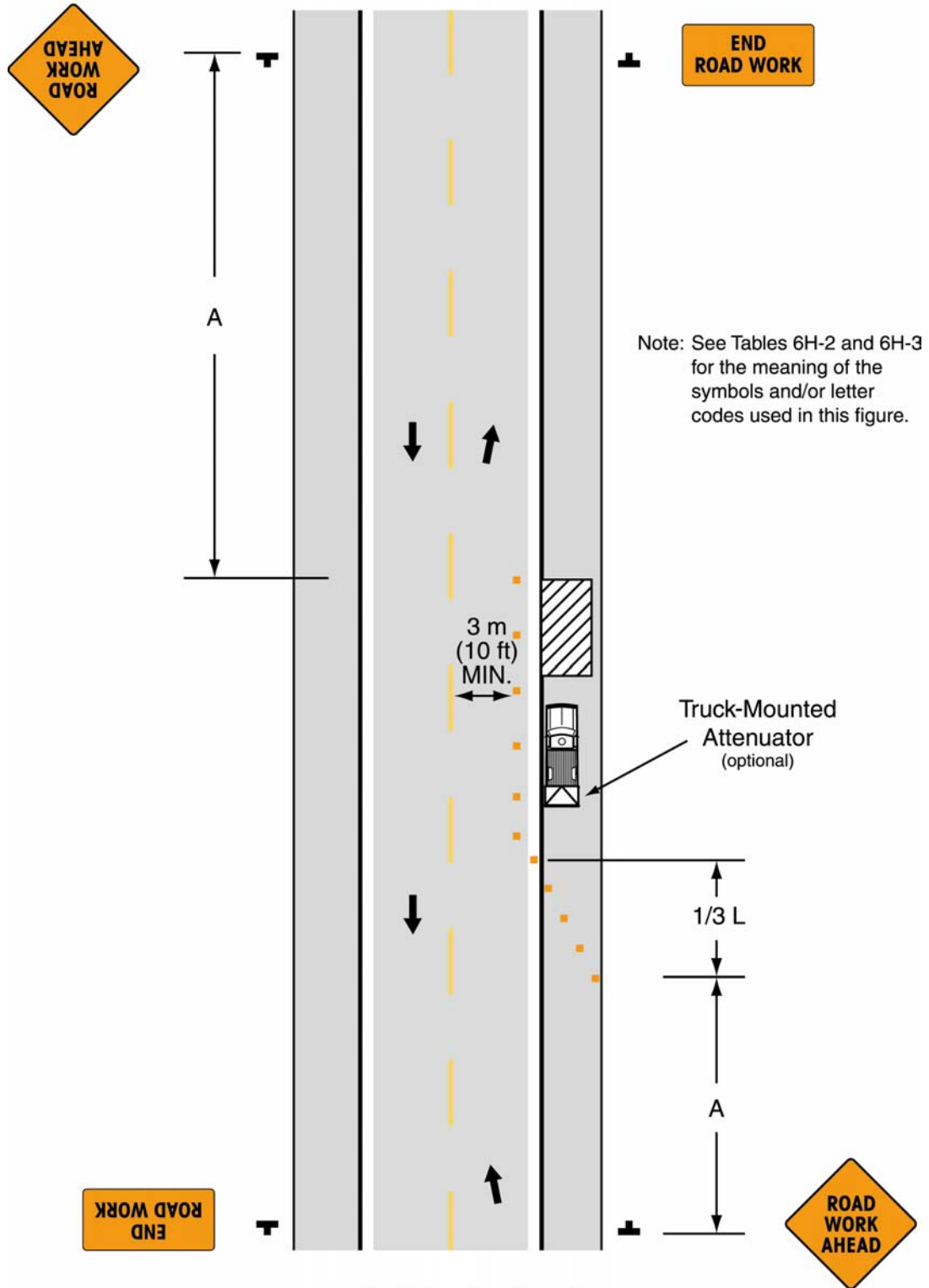
Typical Application 6
