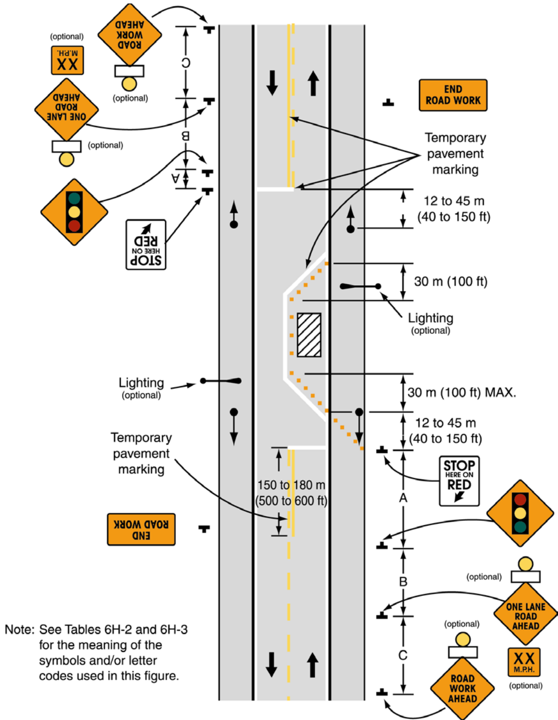
Typical Application 12
