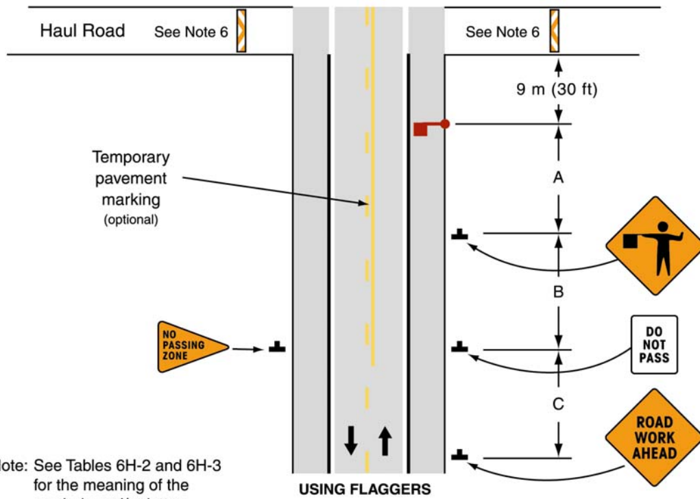
Typical Application 14
