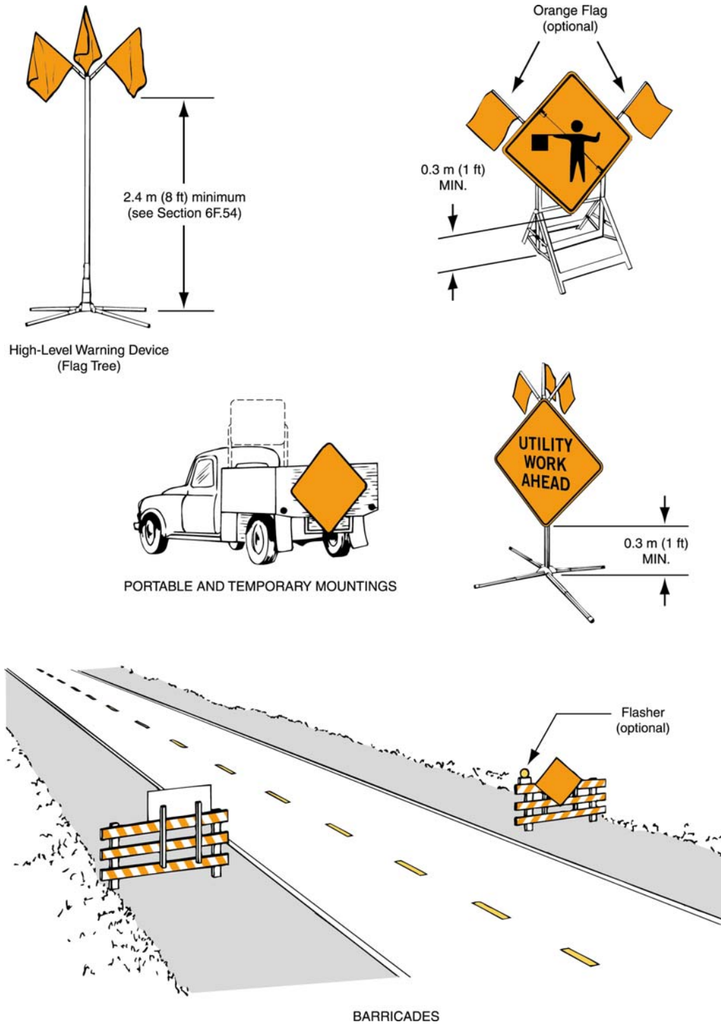
Figure 6F-2. Method of Mounting Signs Other Than on Posts
