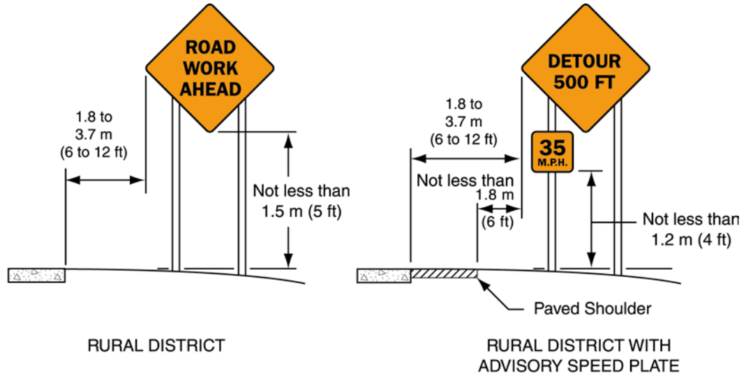
Figure 6F-1. Height and Lateral Location of Signs-Typical Installations
