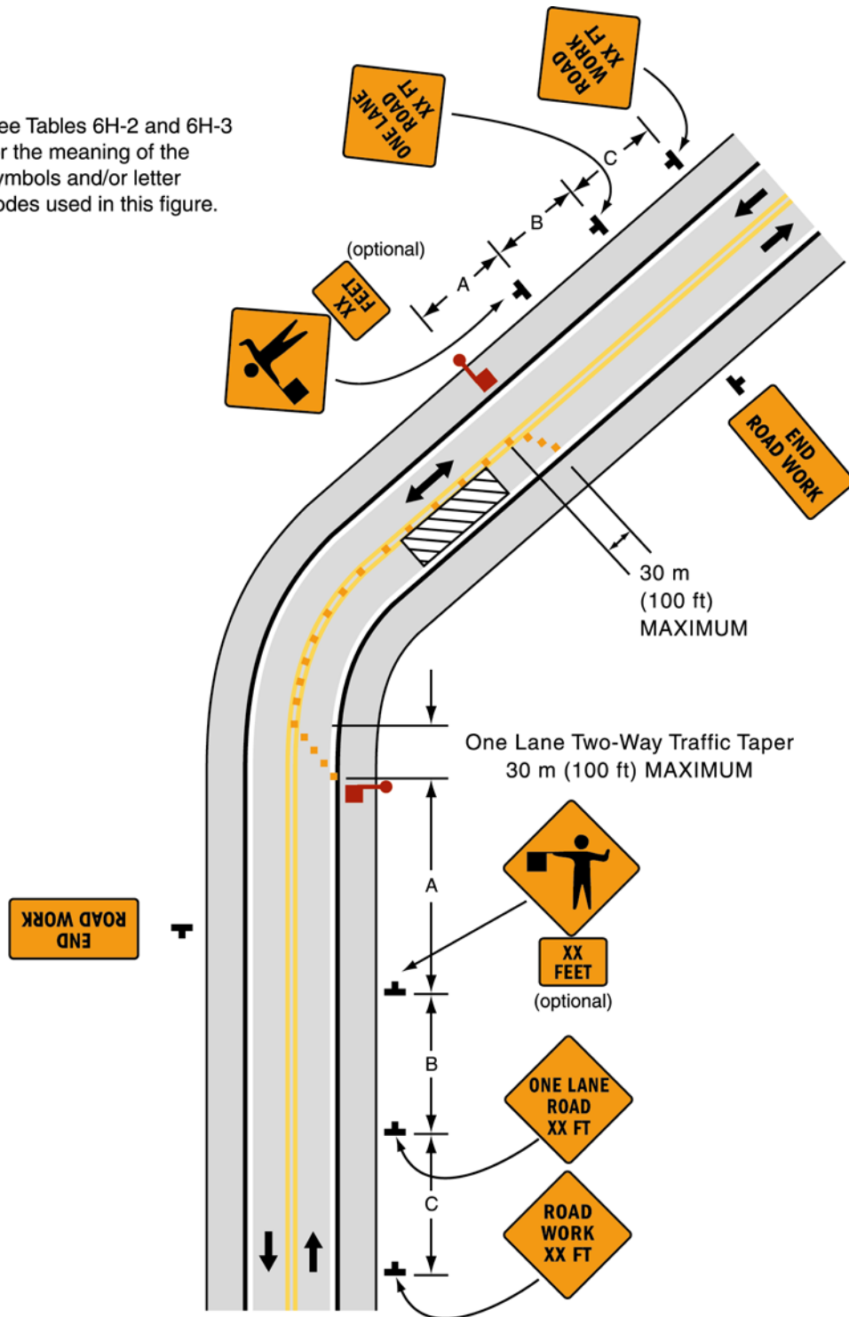
Typical Application 10
