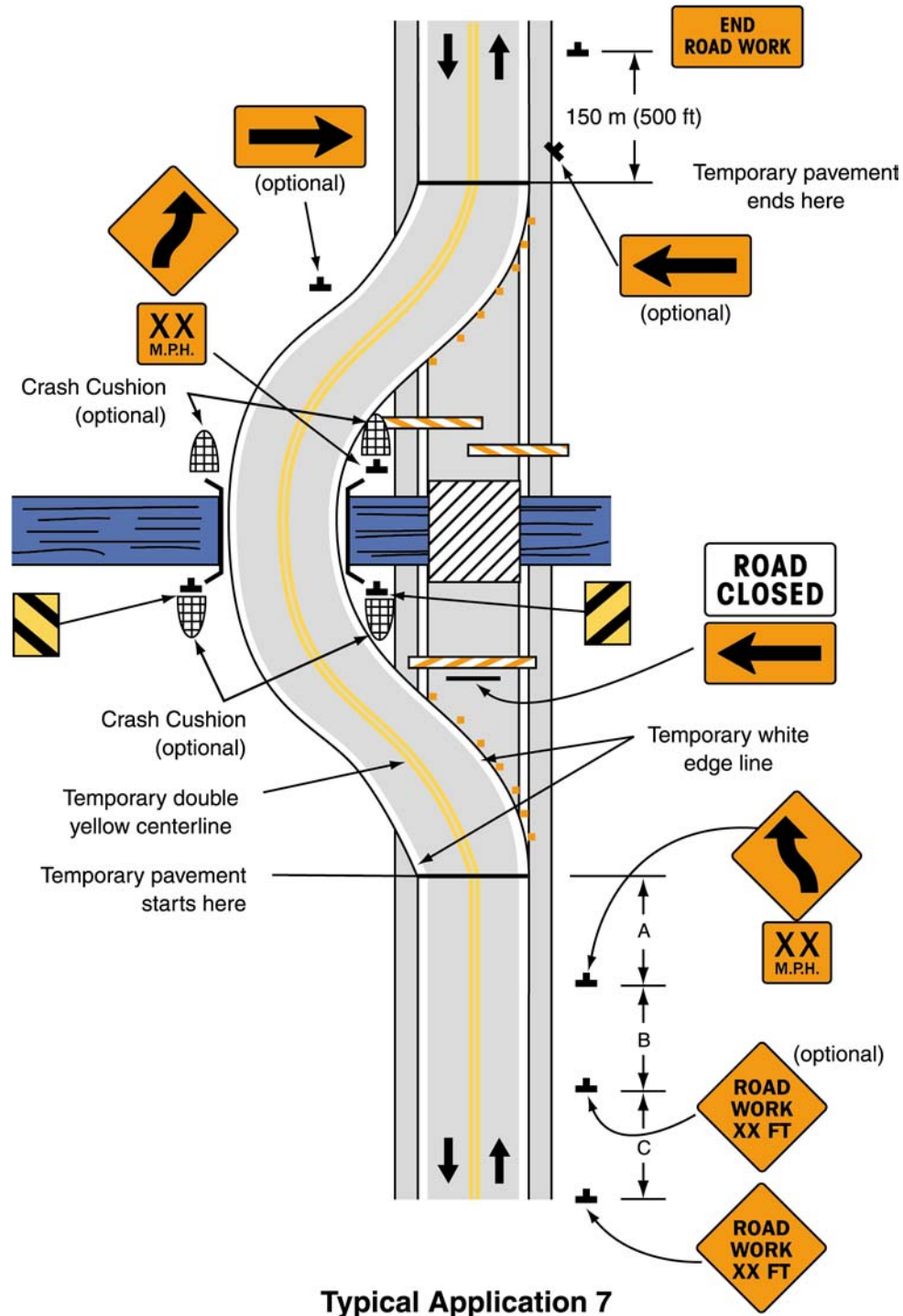
Figure 6H-7. Road Closure with Diversion (TA-7)
