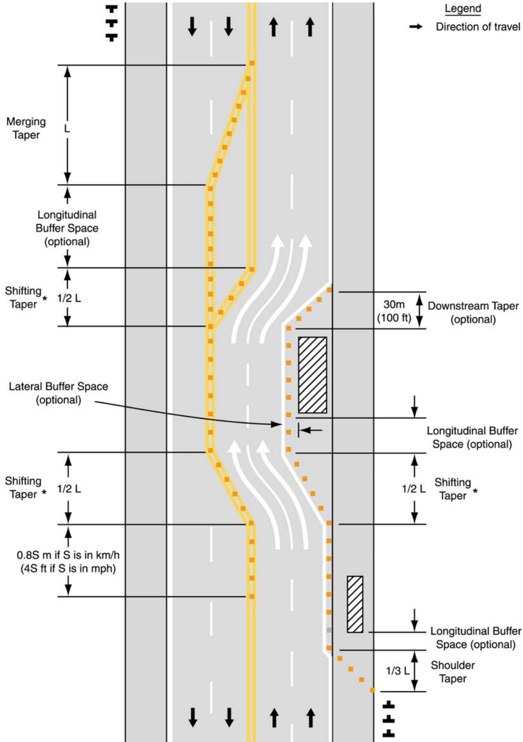
Figure 6C-2. Types of Tapers and Buffer Zones
