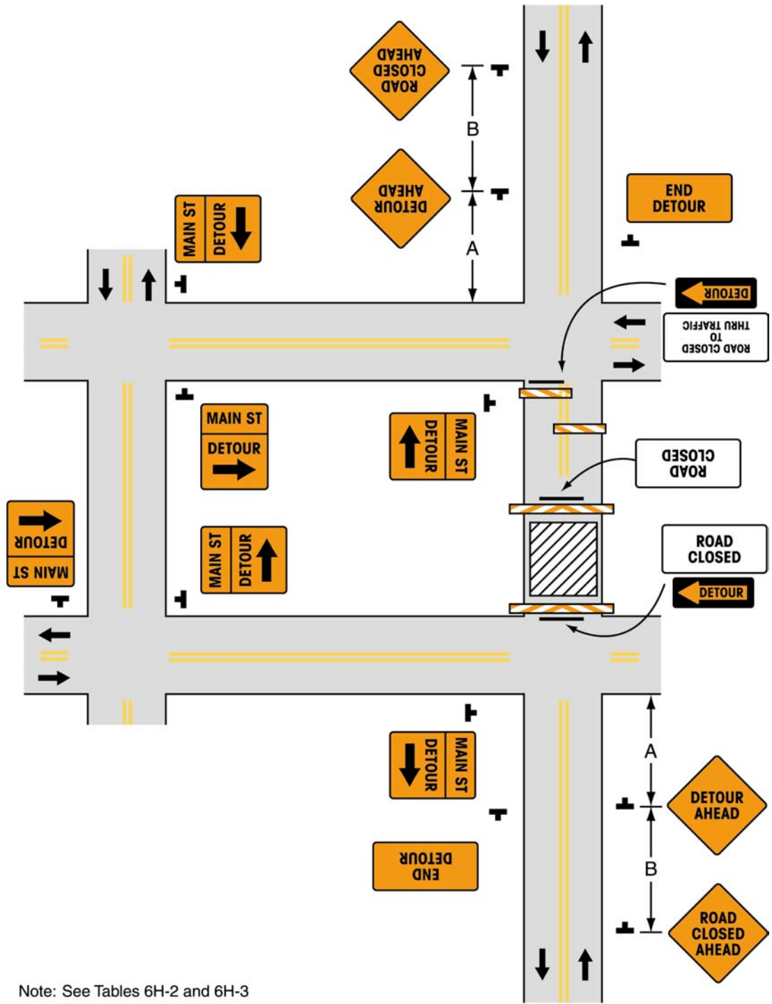
Typical Application 20
