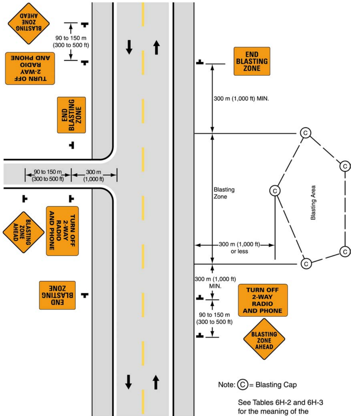
Typical Application 2
