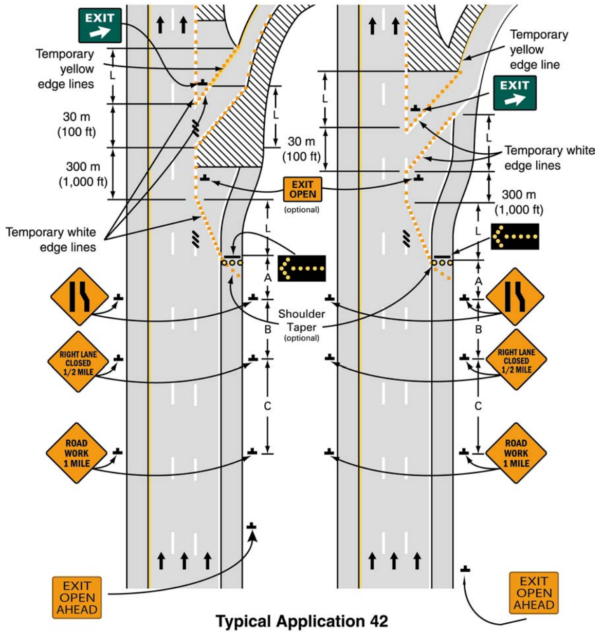
Figure 6H-42. Work in Vicinity of Exit Ramp (TA-42)
