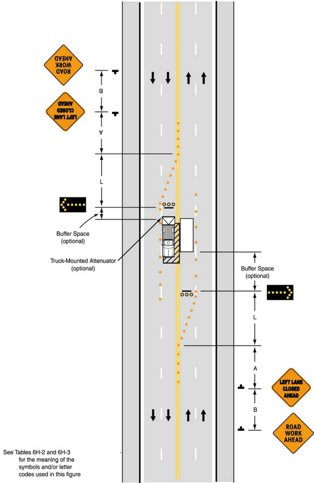
Typical Application 30
