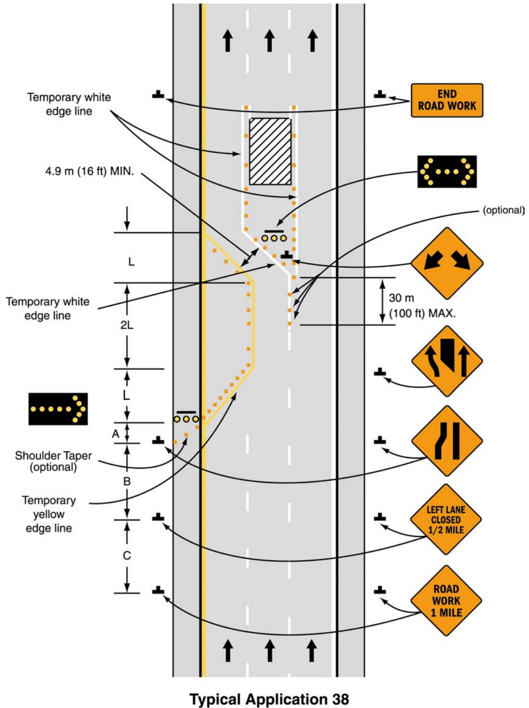
Figure 6H-38. Interior Lane Closure on Freeway (TA-38)
