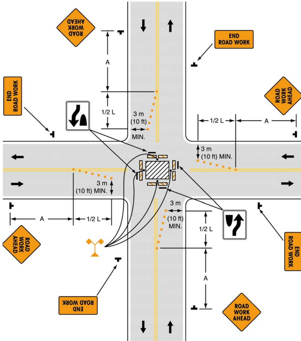
Typical Application 26
