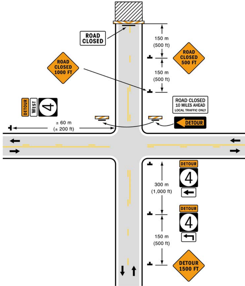
Typical Application 8
