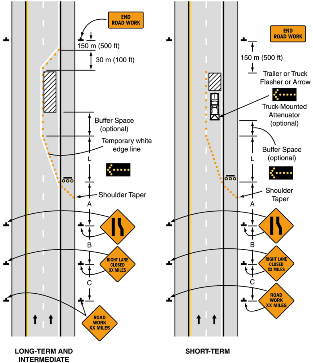
Typical Application 33
