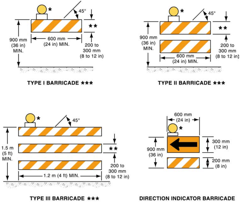
Figure 6F-4. Channelizing Devices (Sheet 2 of 2)
