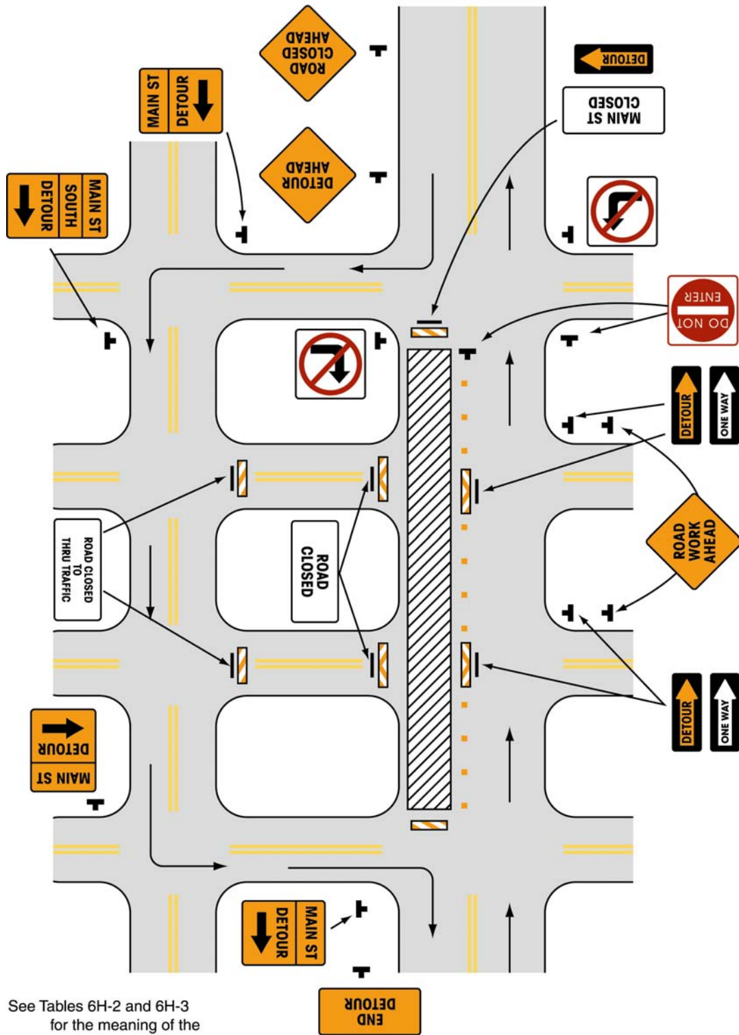
Typical Application 19
