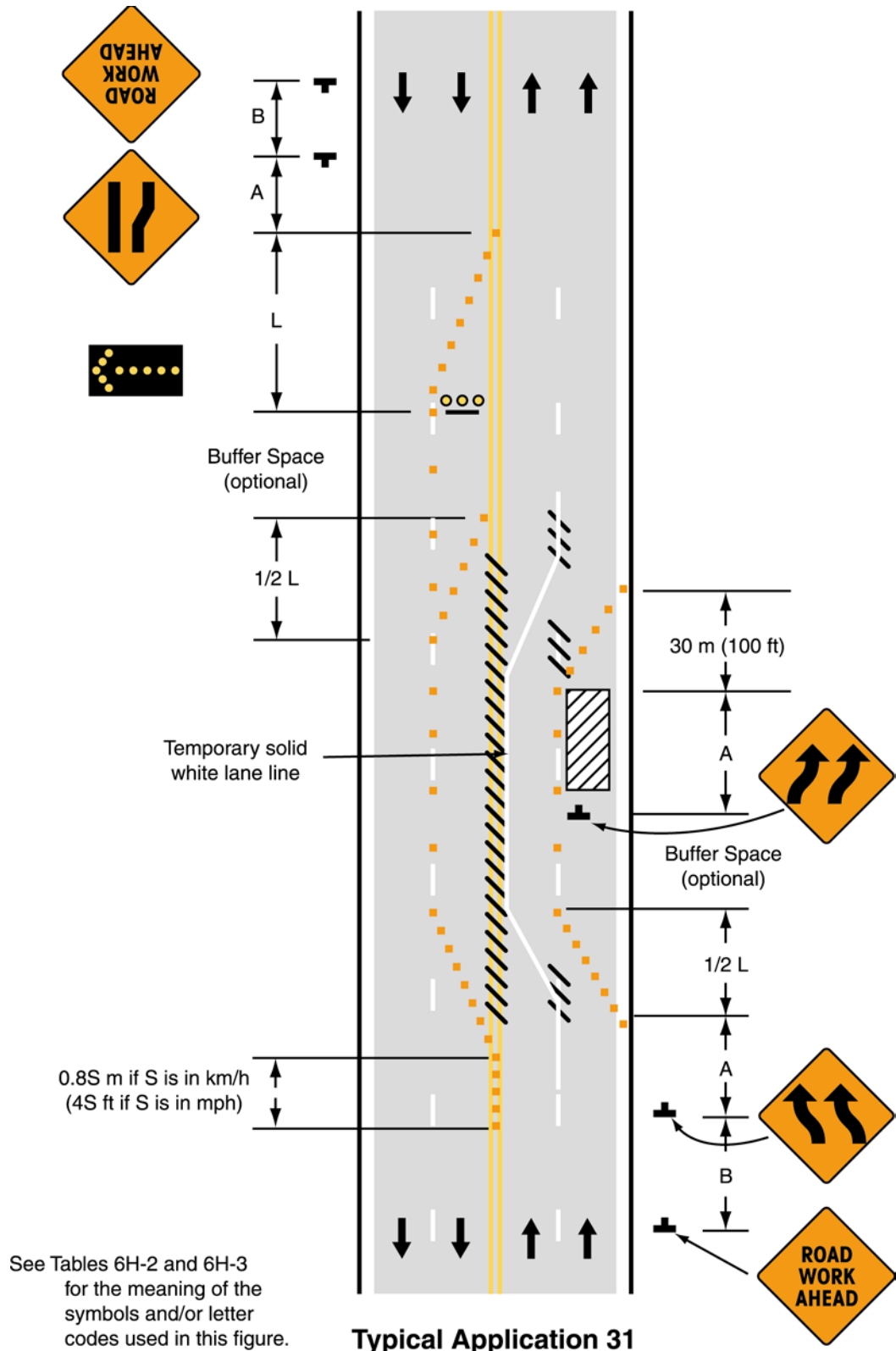
Figure 6H-31. Lane Closure on Street with Uneven Directional Volumes (TA-31)
