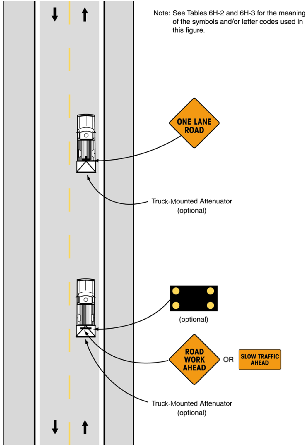
Typical Application 17
