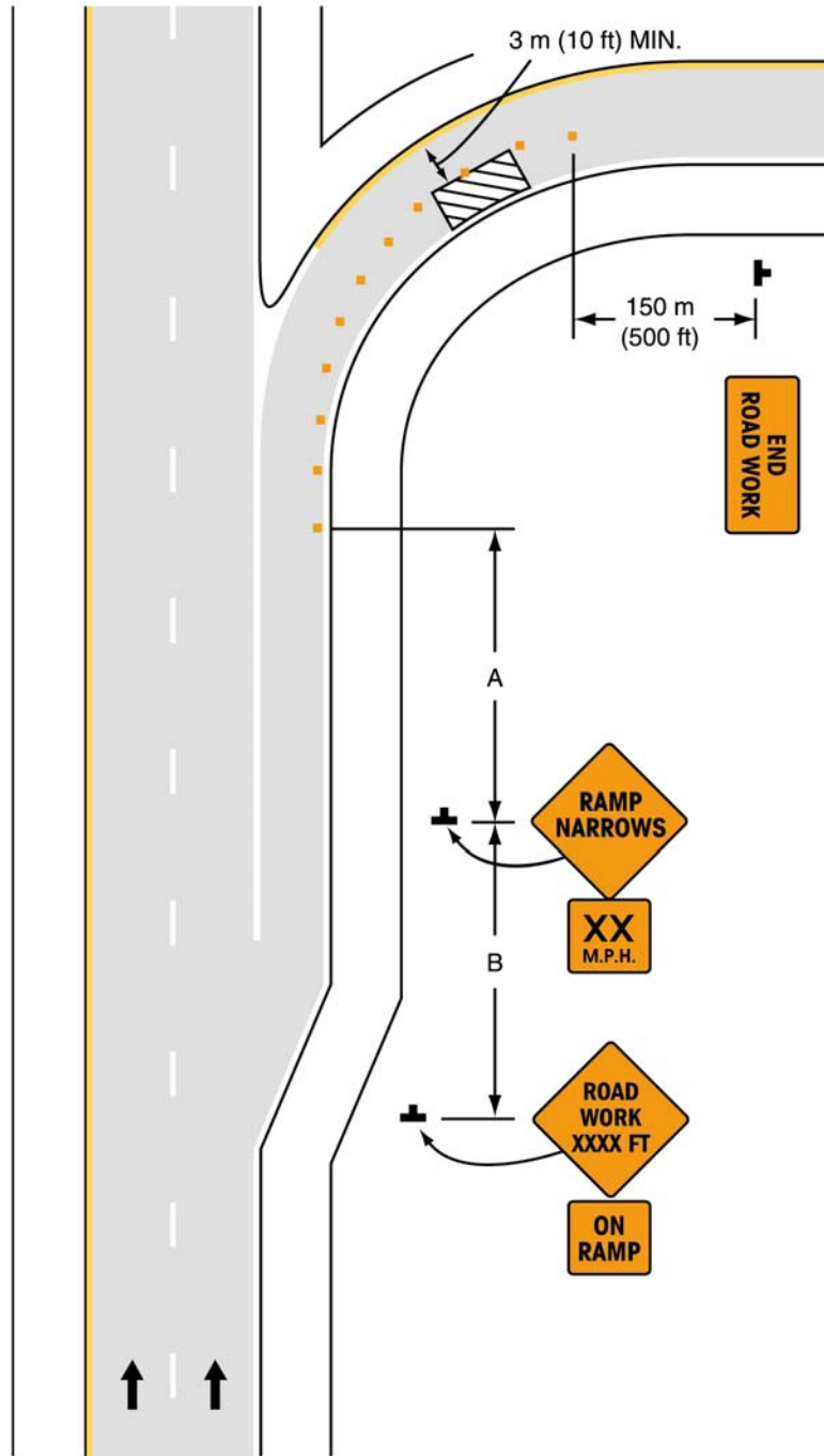
Typical Application 43
