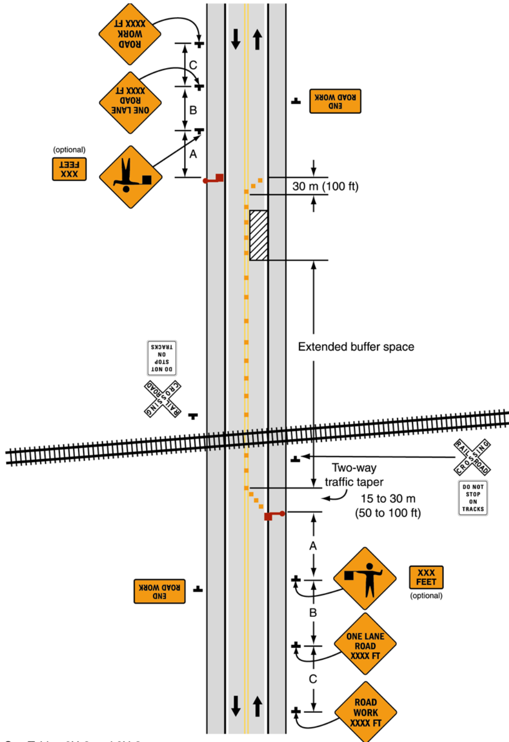
Typical Application 46
