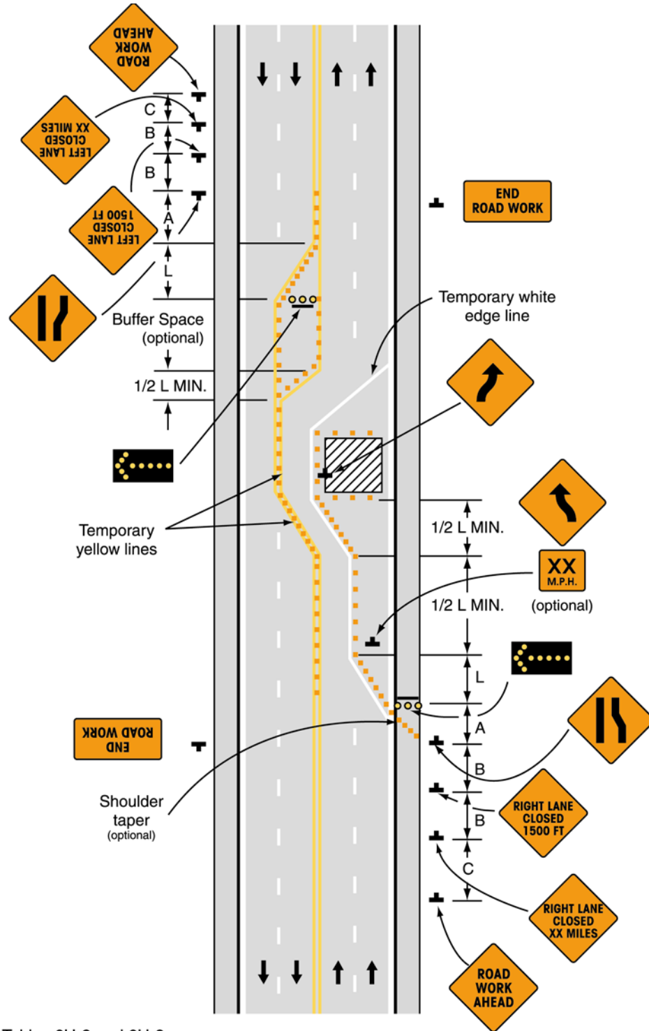
Typical Application 32
