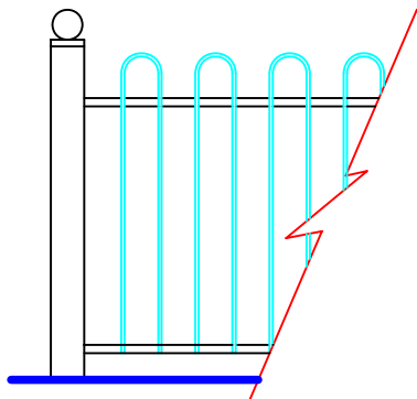
TYPICAL ELEVATION SCALE 1:25
