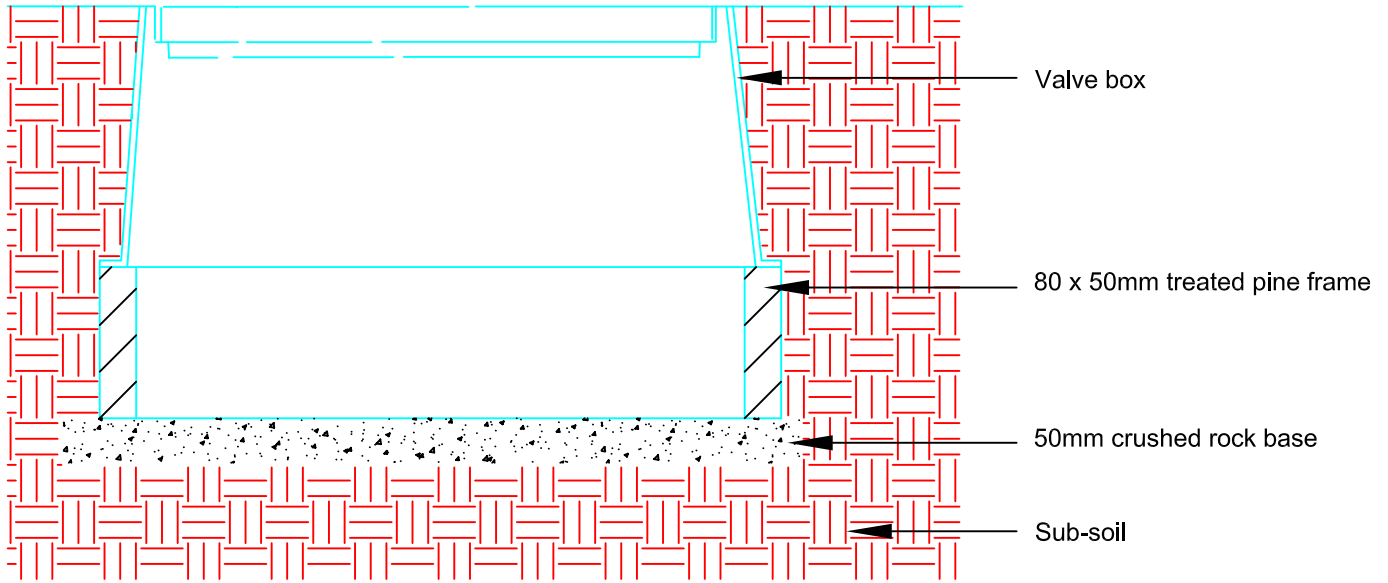
SIDE VIEW
