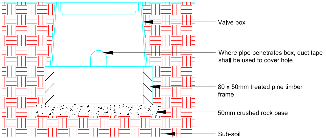
END VIEW
